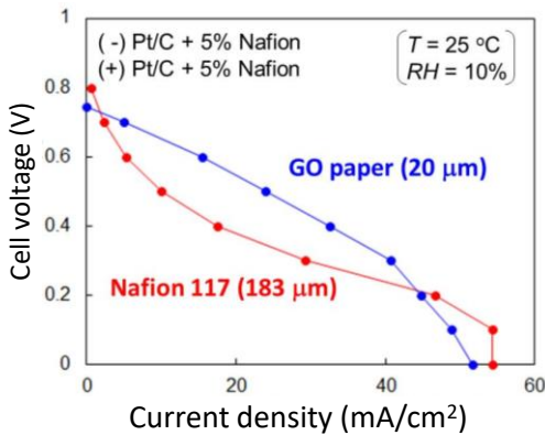
I-V curves
