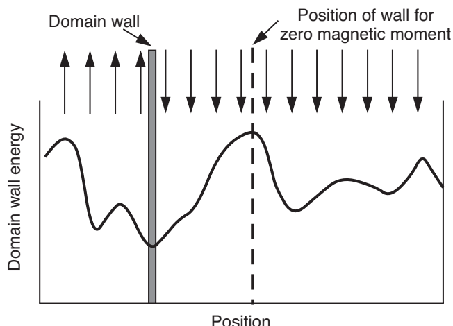
Figure 3.6 Domain wall energy versus position. The solid curve schematically represents domain wall energy; arrows show the direction of j_s within the domains; the domain wall is shown by the stippled region; the position of the domain wall that yields net J = 0 is shown by the dashed line. Redrawn after Stacey and Banerjee (1974).
