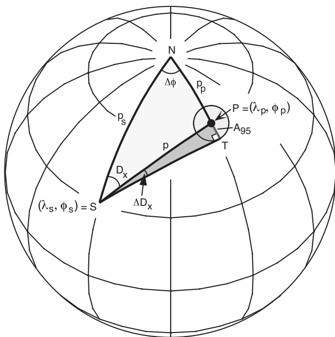
Figure A.5 Geometry used to determine the expected magnetic field direction from a magnetic pole. The magnetic pole is at P (\lambda_p, \phi_p) with circular confidence limit A_{95} ; the site location is at S (\lambda_s, \phi_s) ; N is the geographic north pole; p is the magnetic colatitude of the site; p_s is the geographic colatitude of the site; p_p is the geographic colatitude of the magnetic pole; \Delta\phi is the longitudinal difference between the magnetic pole and the site; D_x is the expected magnetic field declination at the site with confidence limit = \Delta D_x .
